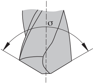
Spitzenwinkel \sigma Point angle \sigma Angolo cuspidale \sigma
