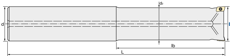
Fig. 1: Steel Shank
