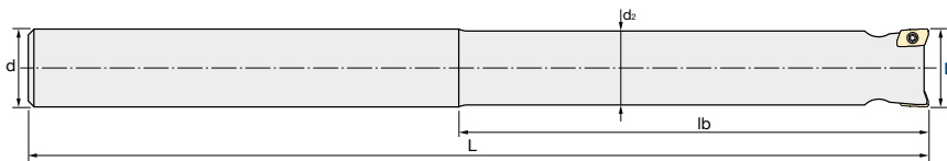
Fig. 2: Carbide Shank
